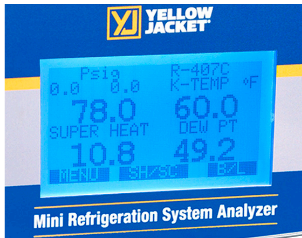
psi - Superheat
