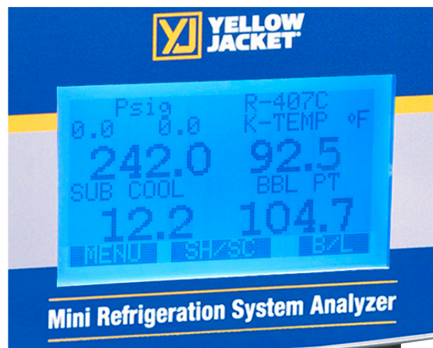
psi - Subcool
